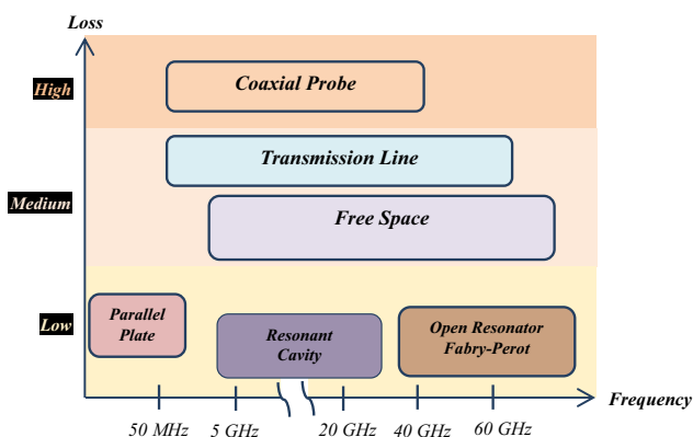
Fig. 2. Summary of dielectric measuring techniques [21].
