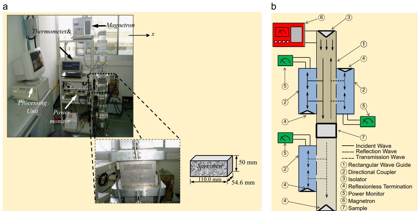
Fig. 7. (a) Experimental set up, (b) schematic showing direction of microwave components (Incident wave, reflected wave, and transmission wave) [46,47].
