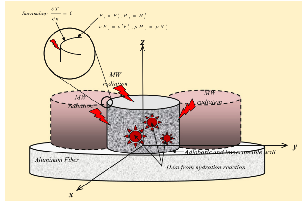
Fig. 11. A physical model and boundary conditions of 0.38-w/c cement paste subjected to microwave energy using a multi-mode cavity [116].
