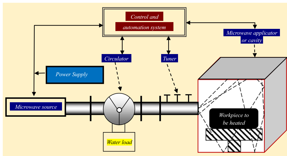
Fig. 6. Microwave system diagram.
