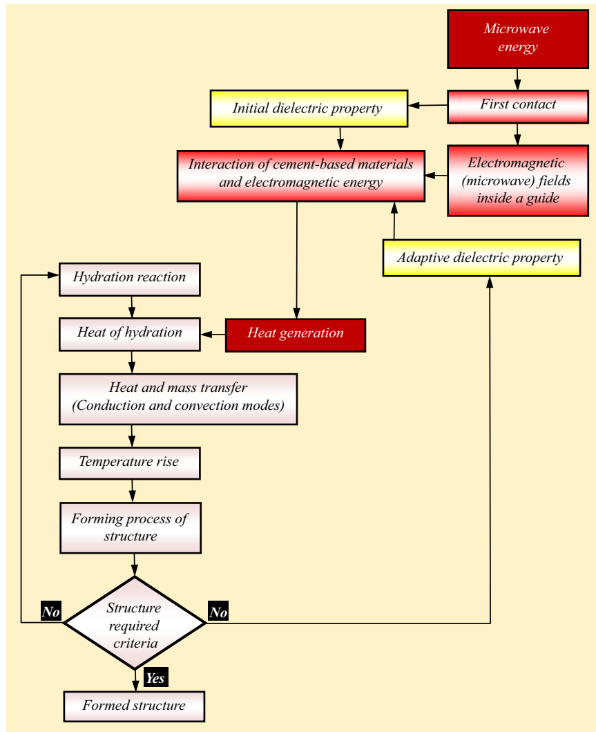
Fig. 12. A proposed schematic model of cement and concrete subjected to microwave energy.
