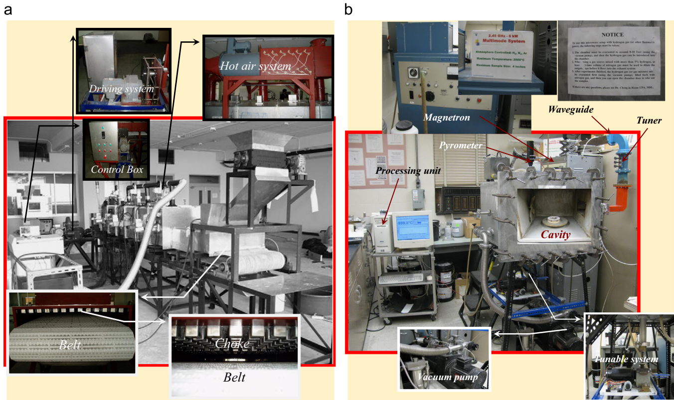
Fig. 8. Microwave system typed multimode resonant cavity: (a) A combined multi-feed microwave-hot air heating with continuous belt system (low temperature multimode microwave system) [48] and (b) high temperature multi-mode microwave system [49].
