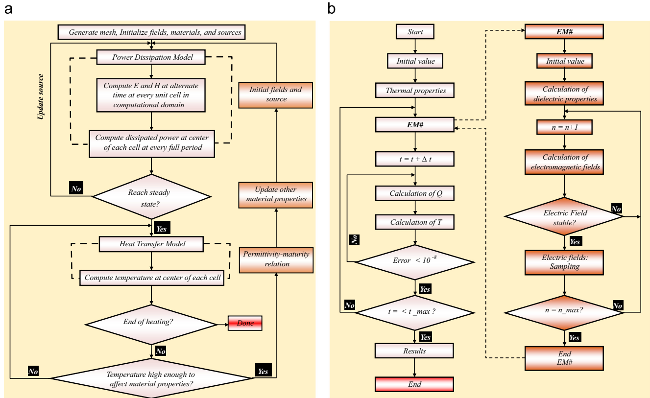
Fig. 10. Microwave heating model. (a) Multi-mode cavity [115] (b) Single mode cavity [46].
