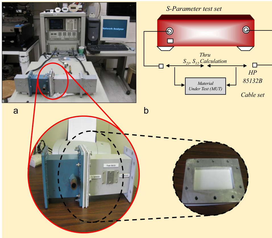
Fig. 3. (a) Network analyzer and (b) schematic of S-parameter test [22].
